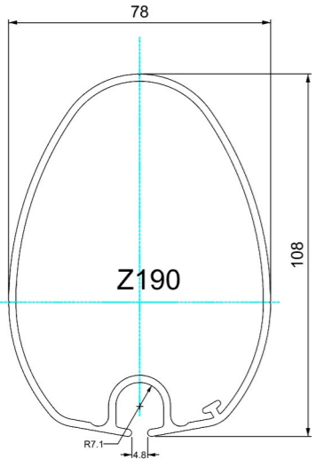
Spar Builder - US Spars (Z-Spars in Europe) Mast Section - Z190 Tack set-up - 60mm Tack set-back - 33mm Gate
